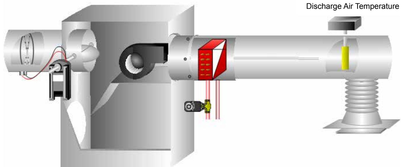
Figure 22: Series Flow Fan Powered Standard Features
