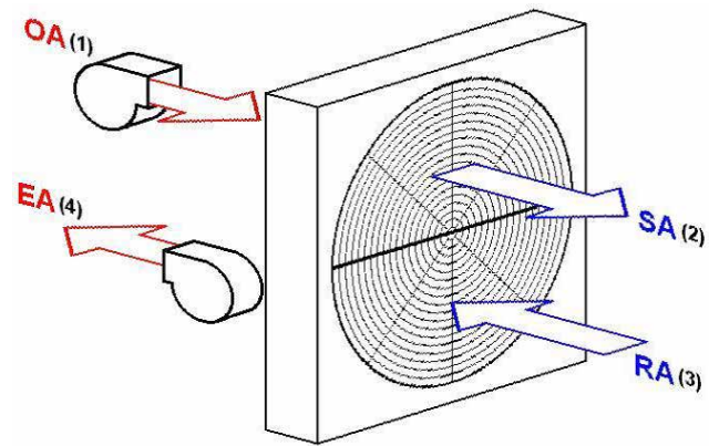
Figure 36: Blow-Thru Supply or Draw-Thru Exhaust
