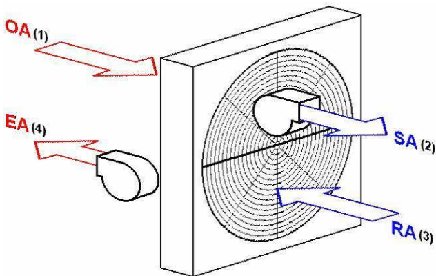
Figure 35: Blow-Thru Supply or Exhaust
